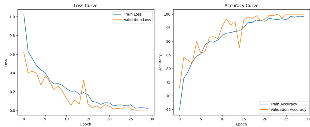
Training and validation learning curves for the custom CNN model.
