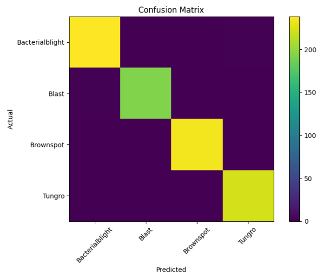
Confusion matrix for the Rice Leaf Disease Classification model.
