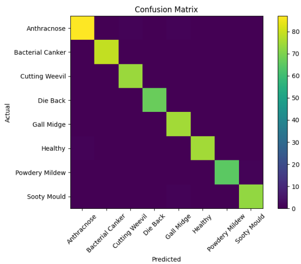
Confusion matrix for EfficientNet-B1 mango disease classification.
