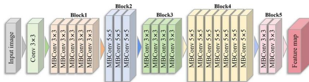
EfficientNet-B1 transfer learning architecture.
