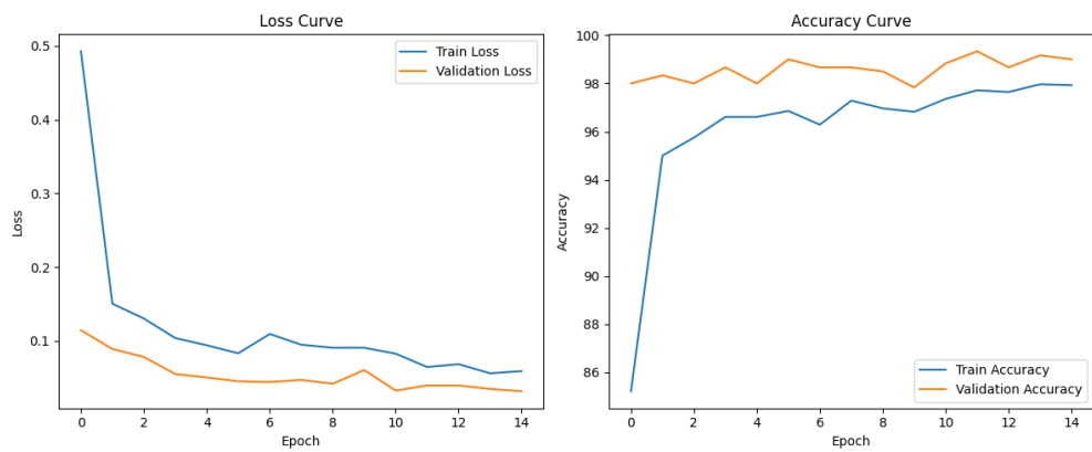
Training and validation learning curves for EfficientNet-B1.
